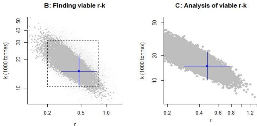
Figure 2. Viable r - k pairs.
