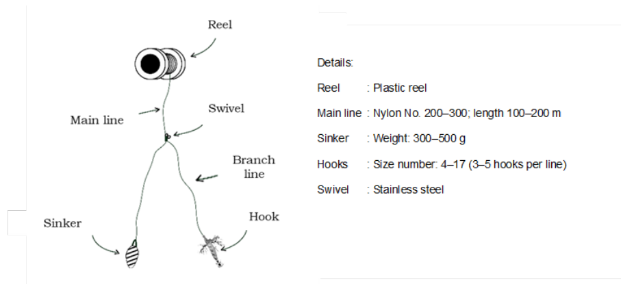
Figure 4. Squid handline construction for fishermen at Sungailiat NFP (Source: Primary data from field documentation, illustrated by the author).
