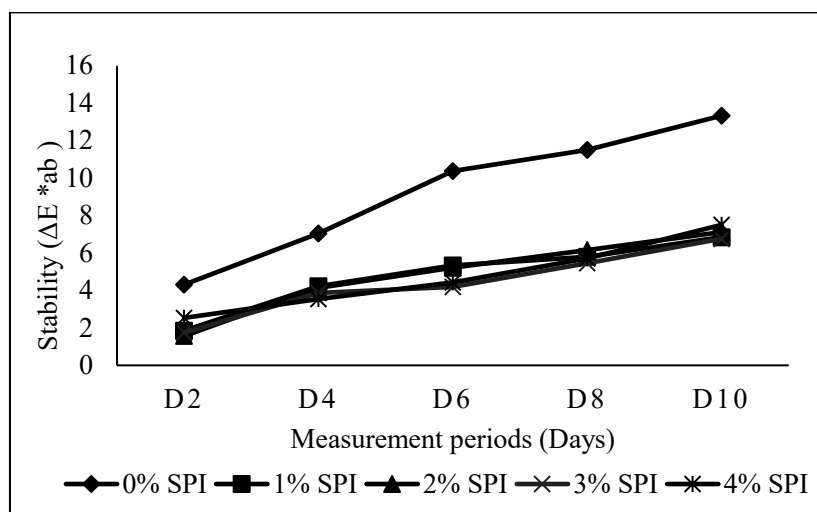
Figure 1. Color stability graph of freshness indicator labels when stored at room temperature (25°C)
