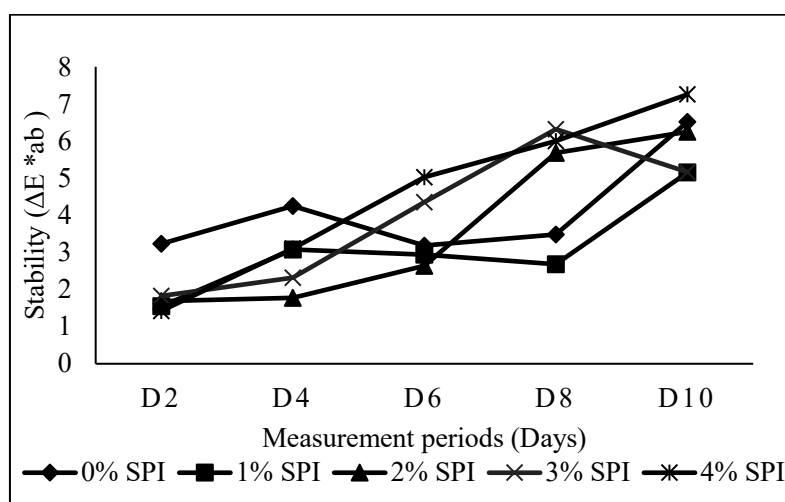
Figure 2. Color stability graph of freshness indicator labels during cold storage (4°C)
