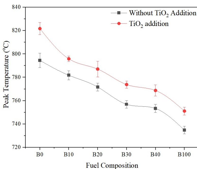
Figure 9. Peak flame temperature.
