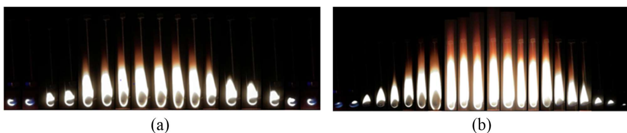
Figure 10. Flame visualization with compositions (a) B0 and (b) B0+ \text{TiO}_2 .
