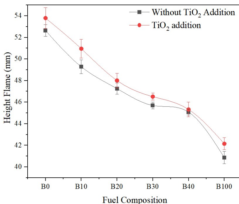
Figure 8. Flame height.
