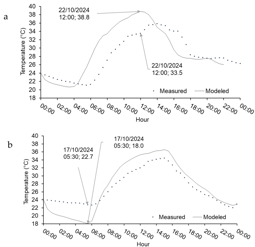
Figure 9. Air temperature inside the greenhouse during extreme maximum outside air temperature (a), during extreme minimum outside air temperature (b).
