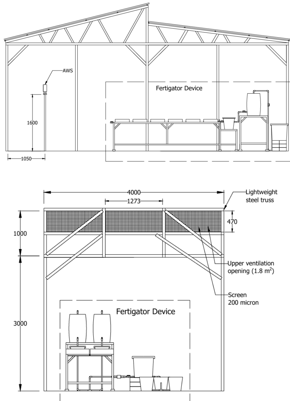
Figure 3. Section A-A and section B-B of the greenhouse.
