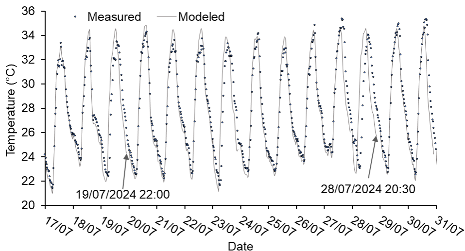
Figure 8. Modeled air temperature and measured air temperature from July 17, 2024 to July 31, 2024.
