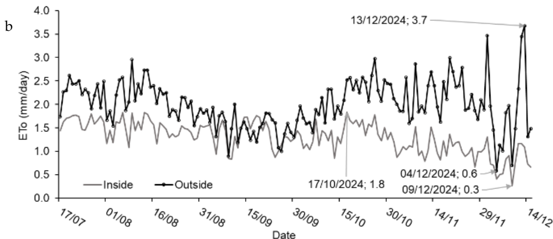
Figure 6. Radiation and rainfall (a), potential evapotranspiration (b).
