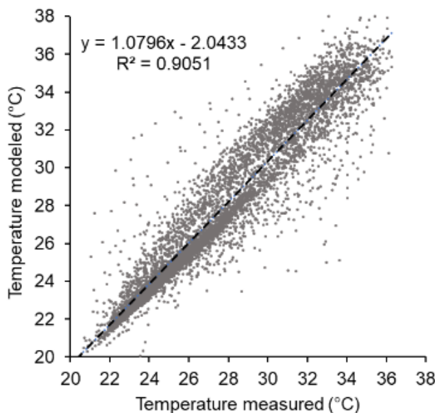
Figure 7. Comparison between measured and modeled greenhouse air temperature.
