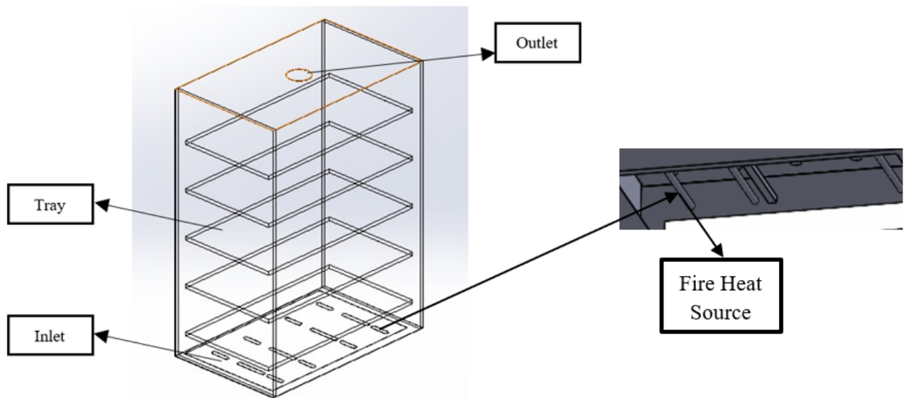
Figure 2. Geometry tray dryer.
