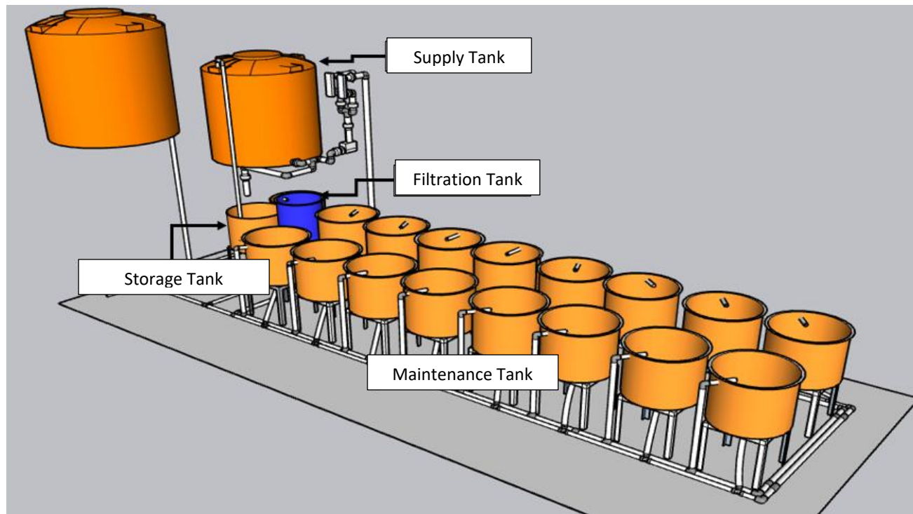
Figure 1. Controlled Water Recirculation System in the Study.
