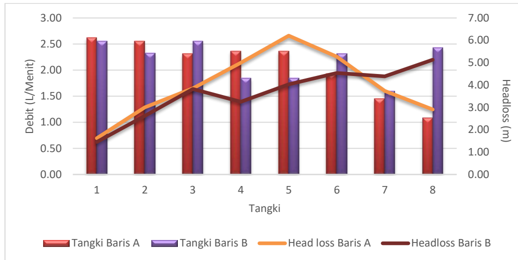
Figure 3. Initial Measurement of Discharge and Headloss.
