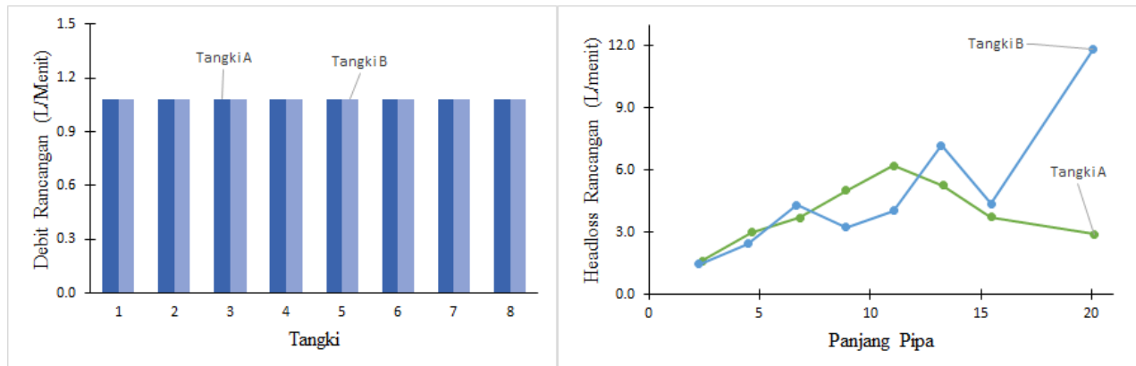
Figure 5. Plan Discharge and Pressure Loss.
