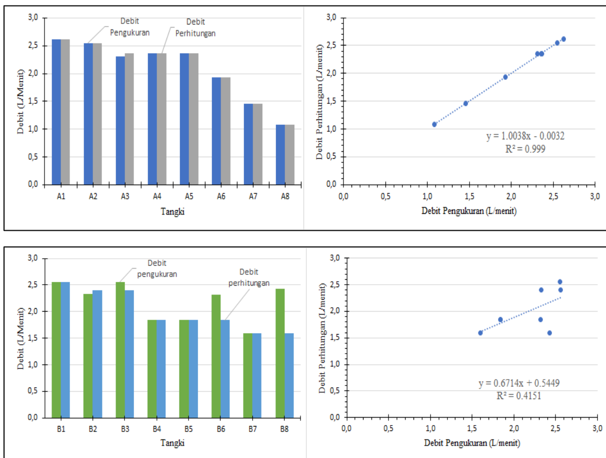
Figure 4. Water balance model analysis and simulation.
