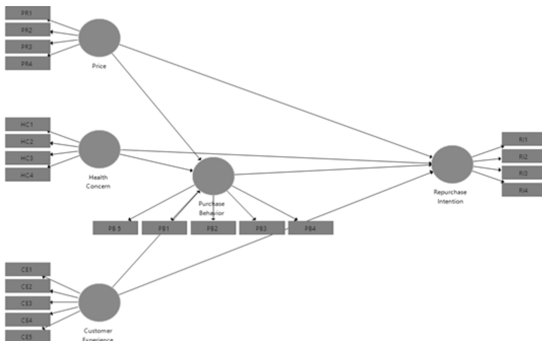
Figure 1 SEM constructs
