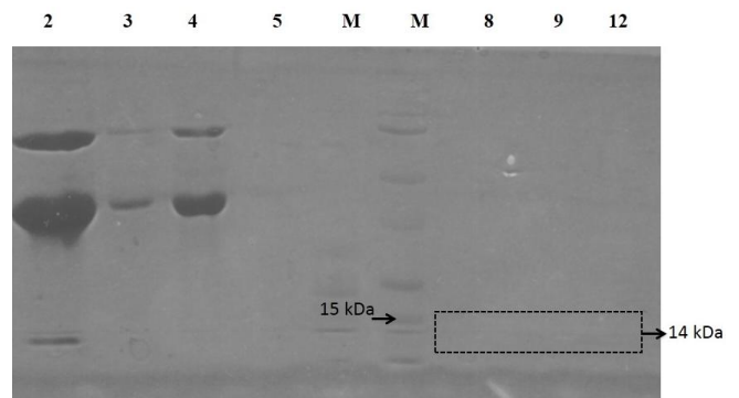
Figure 4B. 15% SDS-Page of purified egg white lysozyme of commercial laying hens using ion exchange chromatography. The number shown in the top of gel corresponds to fraction number in elution profile (4A) in which 10- \mu L aliquotes taken from each respected fraction was loaded into the well.. The bands correspond to lysozyme size are indicated in the dashed box. M lane corresponds to low molecular weight protein markers (Termo Scientific, USA). The marker band corresponds to 15 kD shown in the figure, as it is closed to lysozyme's size. Size label for other bands were omitted for clarity.
