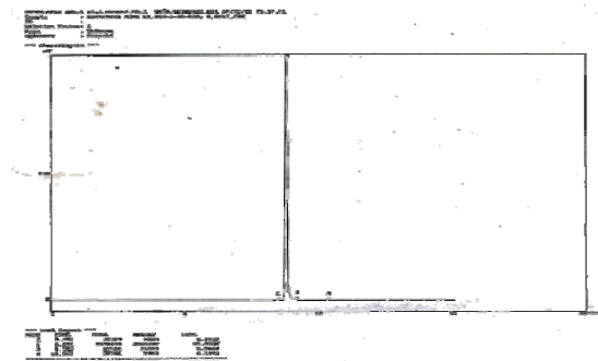
Gambar 2. Kromatogram anetol
