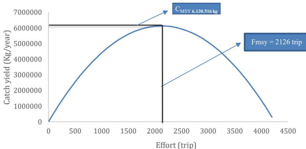
Figure 3. MSY curve of skipjack tuna ( Katsuwonus pelamis ) based on the Schaefer model
