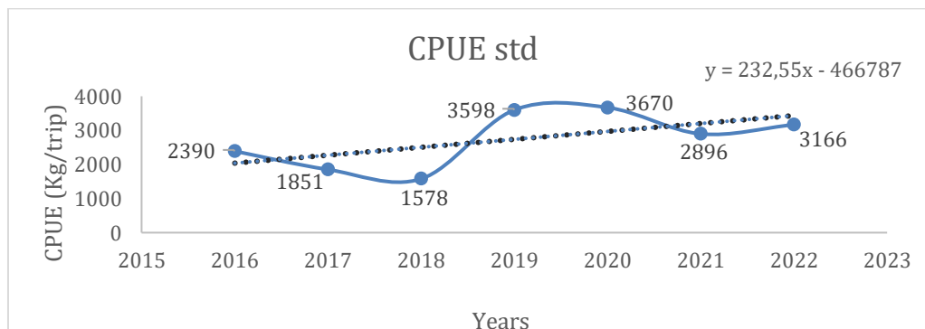
Figure 2. Temporal trend of Catch Per Unit Effort (CPUE) of skipjack tuna ( Katsuwonus pelamis )
