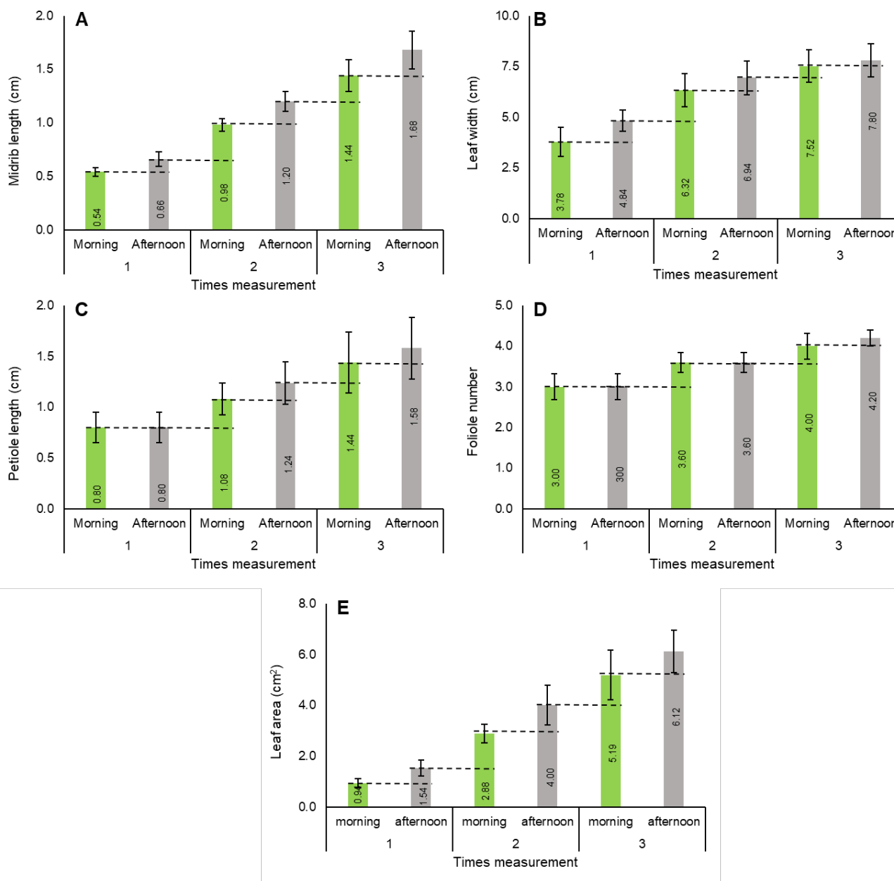
Figure 3. Daily leaf expansion of chikurmanis plant as indicated by midrib length (A), leaf width (B), petiole length (C), foliole number (D), and leaf area (E) in the morning and afternoon. The leaf area was estimated using Y = 0.4964 \times \text{midrib length (M)} \times \text{leaf width (W)} .
