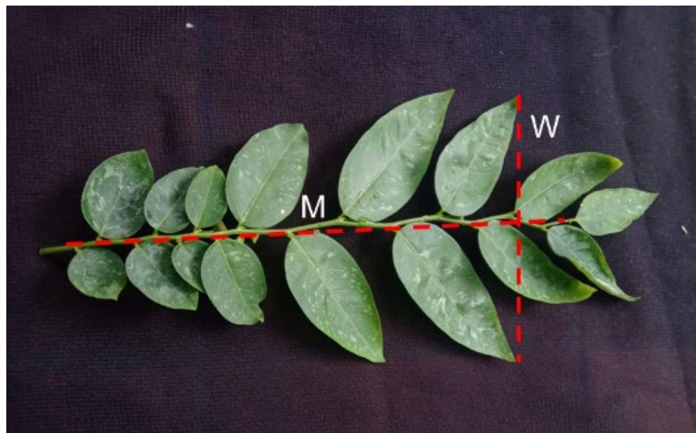
Figure 2. Leaf midrib (M) and leaf width (W) as predictors measured on leaf area estimation.
