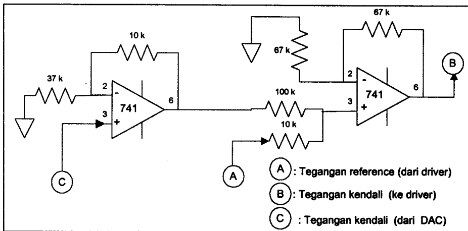
Gambar 3. Signal Conditioner
