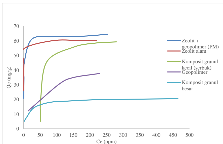
Gambar 5. Kurva hasil adsorpsi metilen biru
