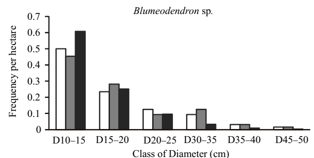
Figure 3 Comparison between stable size distribution from IPMs distribution (■) which is labeled as RELSSD and observed data from time t (□) labeled as REL 2006 in time t to next year (■) labeled as REL 2007 in time t+1 .
