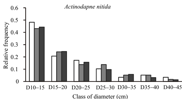
Figure 3 Comparison between stable size distribution from IPMs distribution (■) which is labeled as RELSSD and observed data from time t (□) labeled as REL 2006 in time t to next year (■) labeled as REL 2007 in time t+1 .
