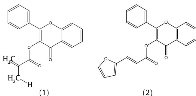
Figure 7. Estimated structure of compounds from LC-MS/MS analysis (1) 3-methacrylate flavonol (tR 8,462) and (2) 3-(furan-2il) acrylate flavonol (tR 9,125)
