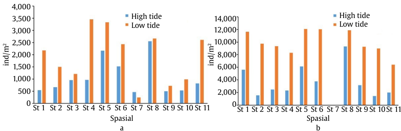
Figure 2. Spatial distribution of Mollusc density during rainy (a) and dry season (b)
