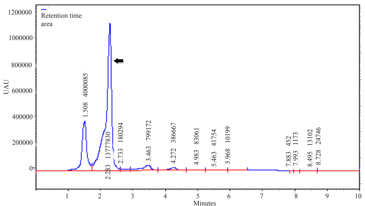
Figure 1. The chromatogram of A. paniculata extract on HPLC analysis. The extract was macerated using 96% ethanol, and injection volume was 1000 ppm. ← Andrographolide.
