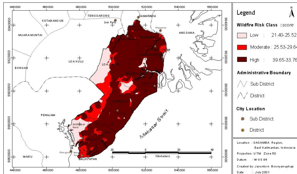
Figure 3. Map of wildfire risk class in the study area
